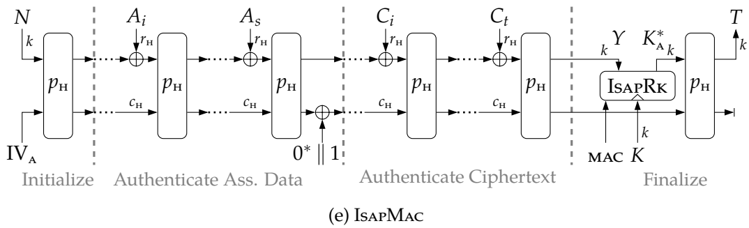
Figure 2.1.: IsAP's encryption \mathcal{E}(K, N, A, M) and decryption \mathcal{D}(K, N, A, C, T) algorithms composing IsAPENC stream encryption, IsAPMAC MAC, and IsAPRk re-keying.
